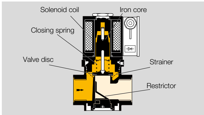
VG 15-40/32..R..N
