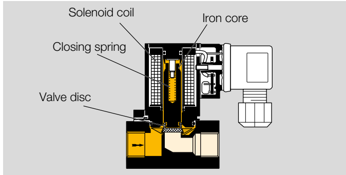
VG 6-15/10..R..N
