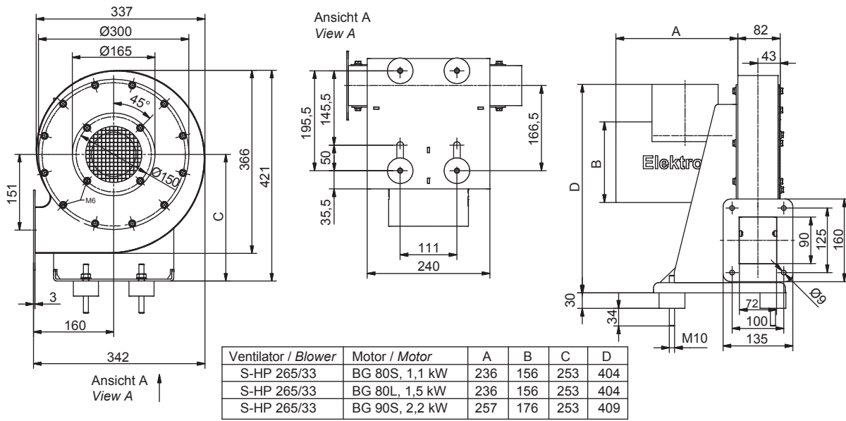
Maße in mm - unverbindlich. Dimensions in mm - subject to modifications.
